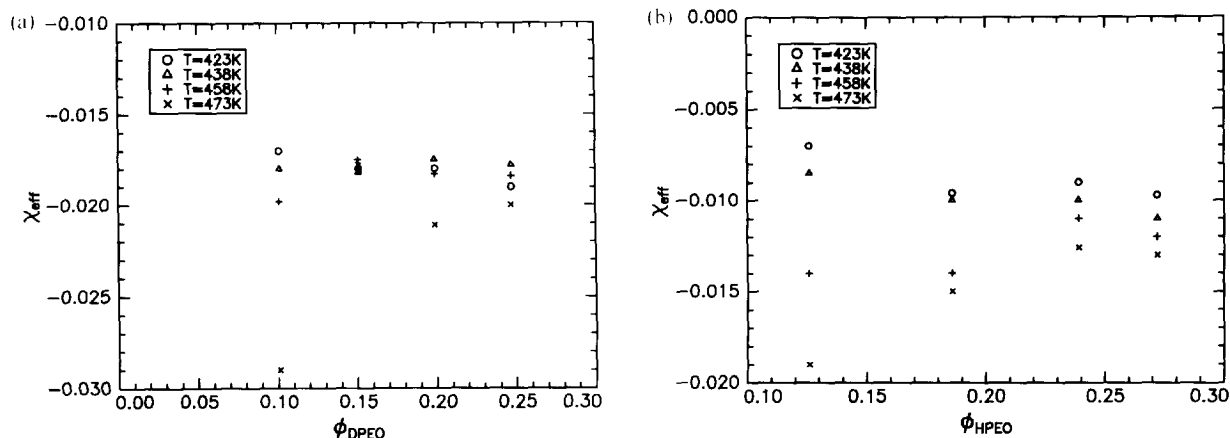
Figure 6 Plots of \chi_{\text{eff}} as a function of polyethylene oxide volume fraction: (a) DPEO-HPMMA blends; (b) HPEO-DPMMA blends
