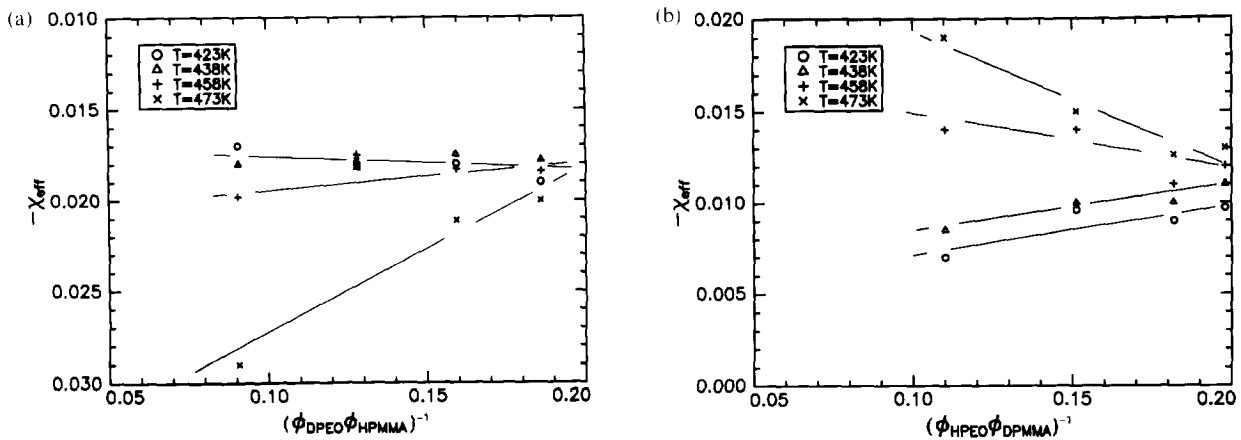
Figure 7 Values of \chi_{\text{eff}} plotted according to equation (9): (a) DPEO-HPMMA blends; (b) HPEO/DPMMA blends. Lines are guides to the eye
